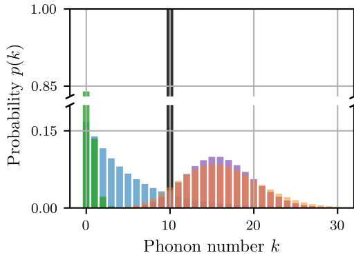
Figure 5.1: Phonon distributions p(k) of a single trapped ion with \omega_y = 2\pi \cdot 2.1 MHz for a thermal state after Doppler cooling (blue), sideband cooling (green) to \bar{k} = 0.2 , Fock state k = 10 (black), a coherent state with \alpha = 4 (purple) and a thermal coherent state after sideband cooling (orange).
