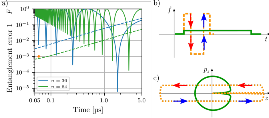
Figure 6.4: a) Entanglement error as a function of gate time (solid) and Rydberg state lifetime (dashed) for states 36P_{1/2} (blue) and 64P_{1/2} (green). b) And c) show the bang-bang electric field control and the trajectory in phase space given by three consecutive kicks (orange) compared to the single square electric field pulse (green). The resulting entanglement error can be reduced to reach the lifetime limit for ultra-short pulse durations as given by the orange diamond in a).
