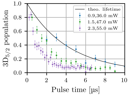
Figure 4.10: Depopulation of the 3D_{5/2} state for Rydberg excitation into 45S_{1/2} as a function of laser interaction time for different laser powers given in the legend as P_{213}, P_{286} . The laser sources deliver sufficient power to drive Rydberg transitions much shorter than the theoretical state lifetime (black), such that coherent population transfer is in reach by future reduction of the excitation linewidth.
