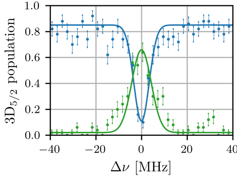
Figure 4.5: 55\text{S}_{1/2} excitation spectrum probed by residual population in the 3\text{D}_{5/2} state as a function of two-photon detuning \Delta\nu for direct excitation (blue) and the QI method (green). Error bars depict the quantum projection noise and solid lines are Gaussian fits to the data to extract transition frequency and linewidth, where the full width at half maximum is 7.9(7) MHz for the direct excitation spectrum and 10(9) MHz for the QI spectrum.
