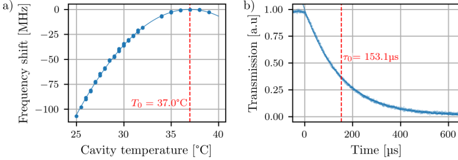
Figure 3.5: a) Measurement of the zero expansion temperature T_0 by varying the cavity temperature and measuring the atomic 3D \rightarrow 5P transition with the fundamental beam at 852 nm locked to the high finesse cavity. b) Ring-down measurement of the light field inside the cavity with decay constant \tau_0 to estimate the finesse.
