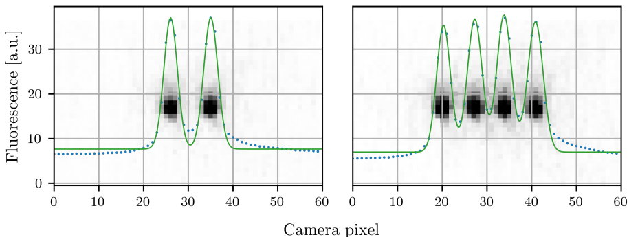
Figure 7.2: Fluorescence images to extract the imaging magnification of the experimental setup with a two-ion crystal at center-of-mass mode frequency \omega_z = 2\pi \cdot 0.54 kHz (left) and consecutive determination of interparticle distances in a four-ion string within the same trap potential (right). Blue data points are integrated fluorescence counts along columns of the presented crystal image with Gaussian fits in green.
